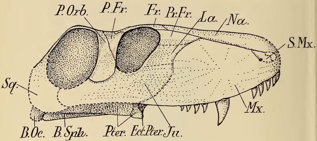
FIG. 12.— Cynariops robustus . Type. Lateral view of the skull. \times \frac{1}{4} .
